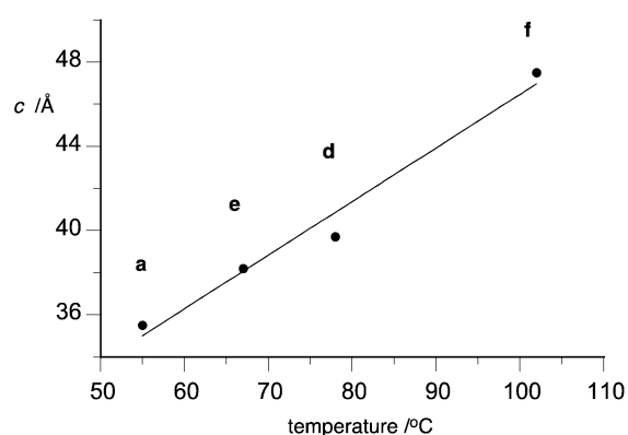
Fig. 8 A correlation between the Col h(3D) –I (Col h(3D) –Col h ) transition temperature and the lattice parameter c for 1[10]d .
