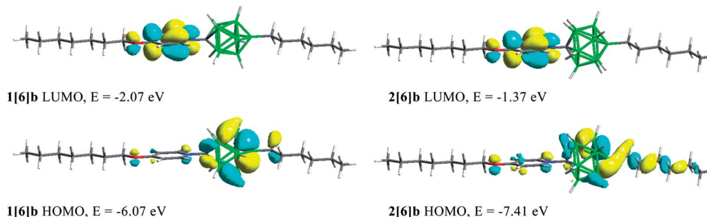
Fig. 3 B3LYP/6-31G(d,p) derived contours and energies of FMOs involved in low energy excitation in 1[6]b (left) and 2[6]b (right).
