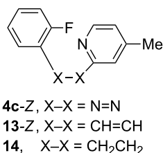
Figure 6: Structures of three close analogues.
